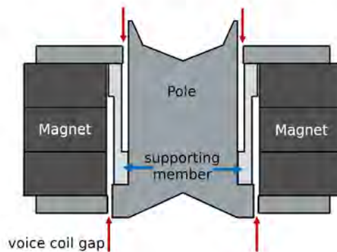
Figure 4. Schematic of the Uni-Core driver motor
