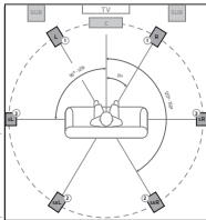
SPEAKER PLACEMENT IN LISTENING AREA
