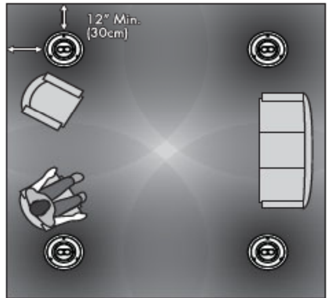
Figure 13. Helos 22: Wide dispersion. Mono mode used for distributed audio.
