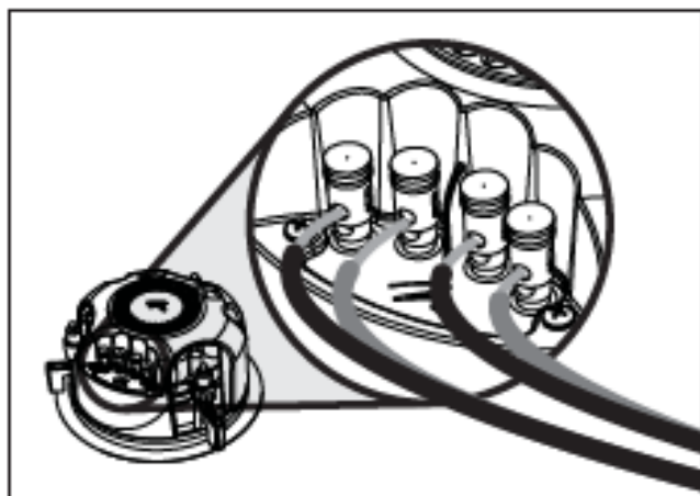
Figure 2. Connecting the Helos 22 for stereo use.
