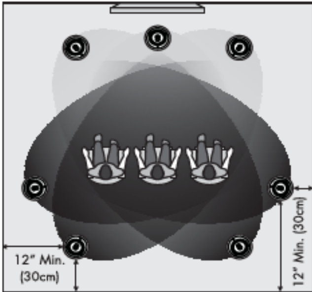
Figure 6. Helos 12: Adding surround channels to create a 5- or 7-channel installation.
