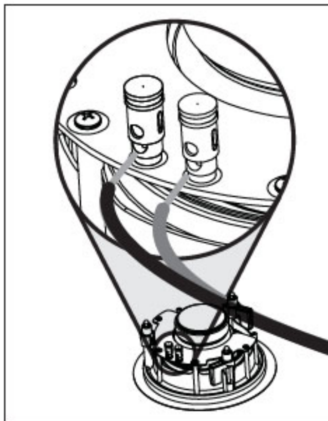
Figure 1. Connecting the Helos 12.
