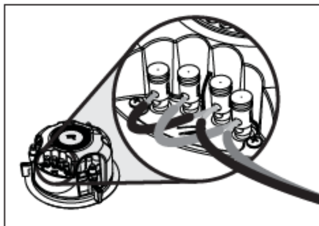
Figure 3. Helos 22 bridged for mono use.
