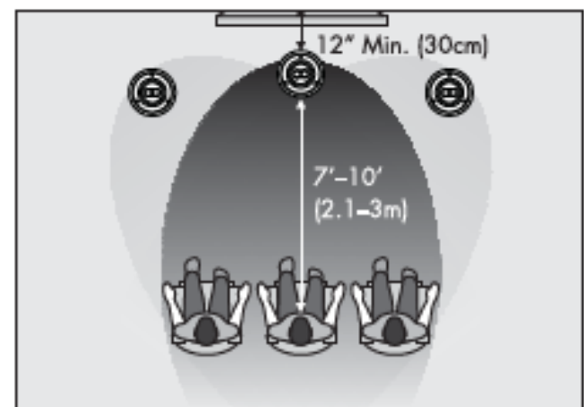
Figure 5. Helos 12: Adding a center channel.
