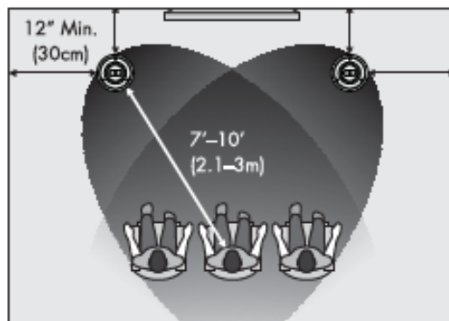
Figure 4. Helos 12: 2-channel installation.
