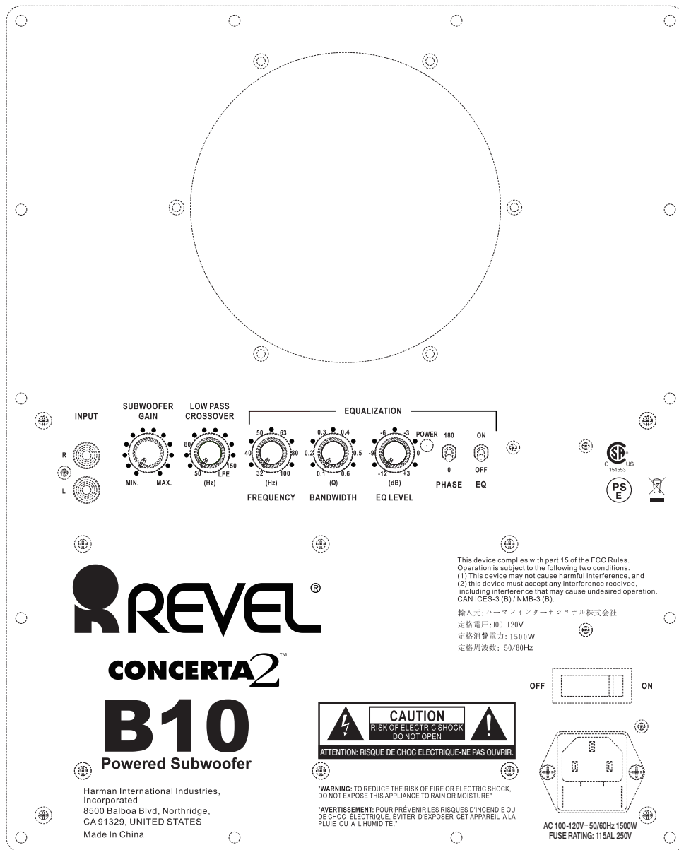
Figure 14: Rear-panel controls and connectors
