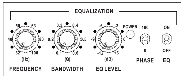
Figure 18: Equalization controls
