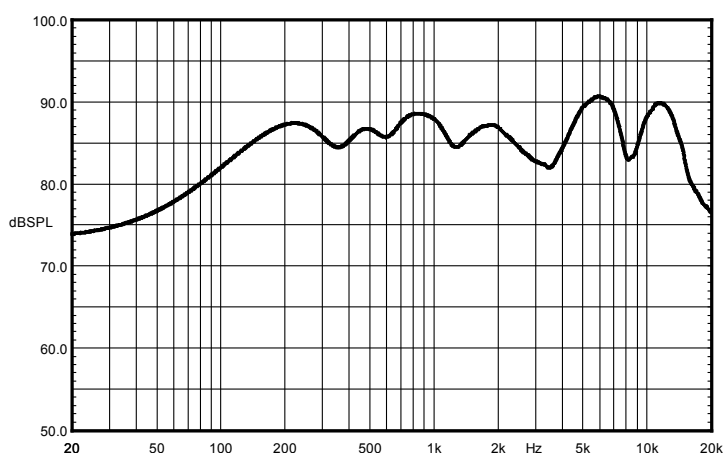
SAROS IC8T – Frequency Response
