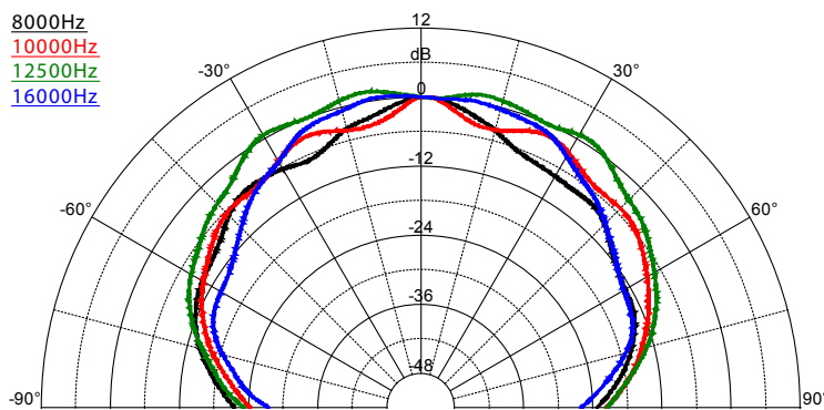
SAROS IC8T – Dispersion Pattern, 8000 Hz - 16000 Hz
