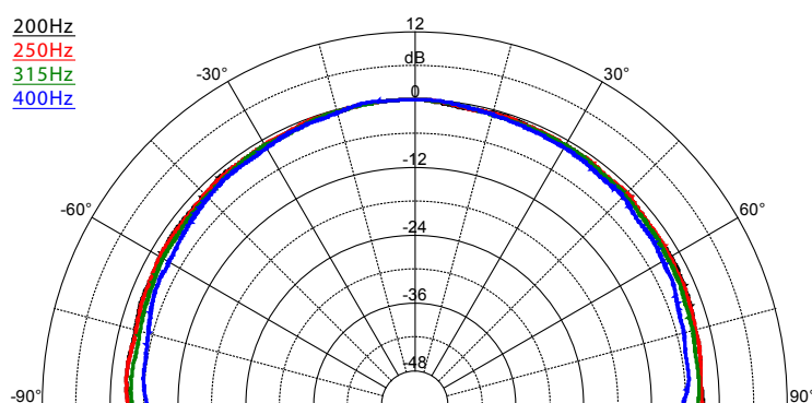
SAROS IC8T – Dispersion Pattern, 200 Hz - 400 Hz
